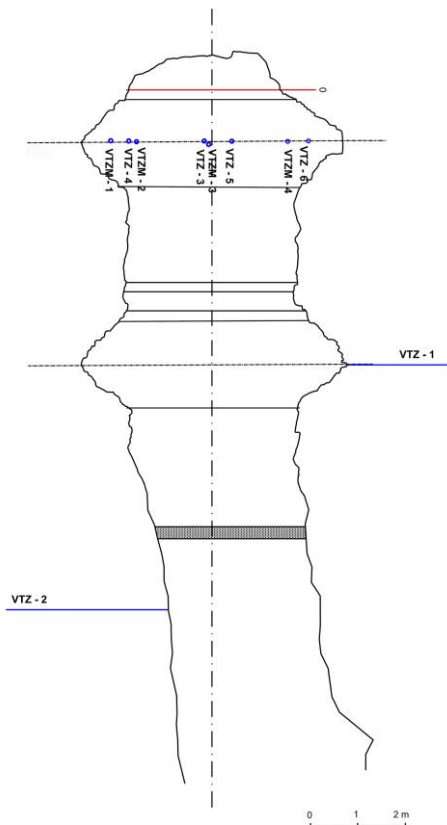
Figure 2 Location of the tested boreholes (WPT in the SP-59 niche)(Záruba, 2015)
