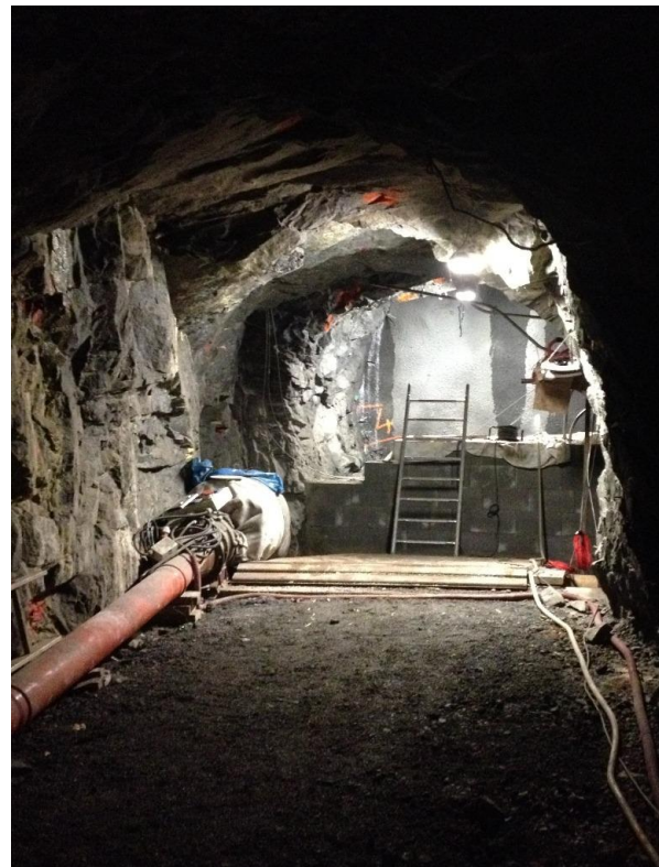
Figure 4 Grouting work in the SP-59 niche
