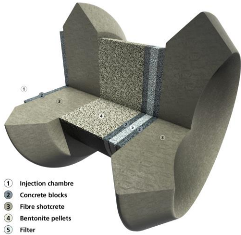
Figure 1 Cross-section through the plug
